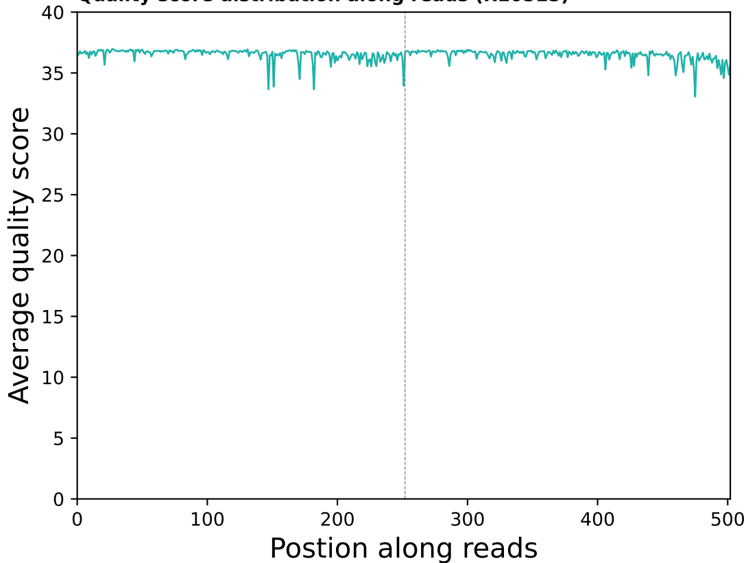
Quality score distribution along reads (R10515)
